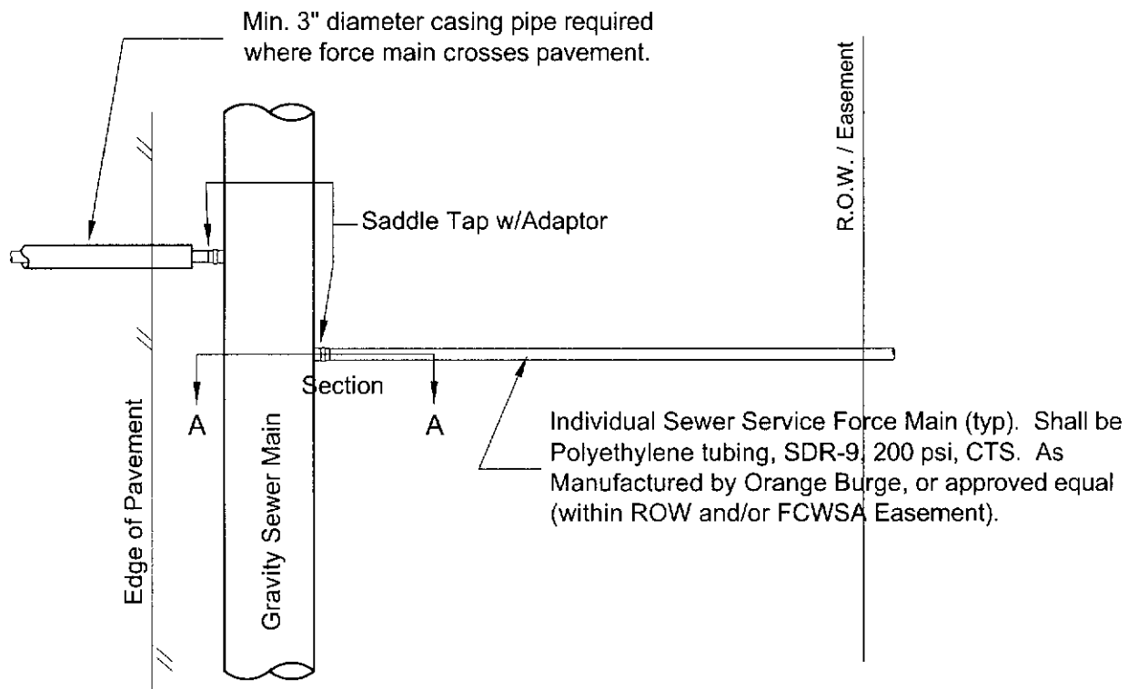
Typical Private Force Main Connection (NTS)
