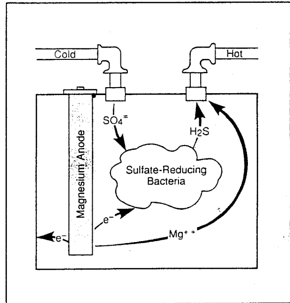
Figure 1 Bacterial action in water heater.
